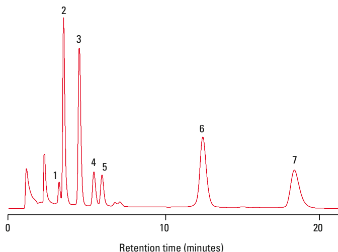
FIGURE 11 Separation of Tetracycline
